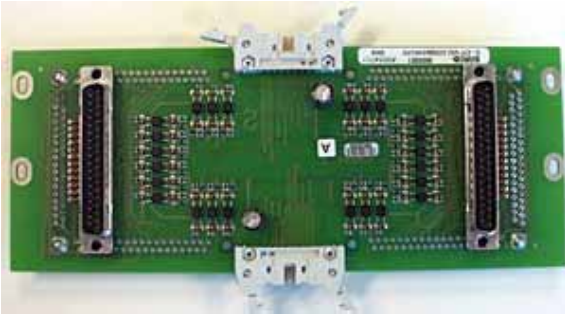
A505471 - Q-stop board ACO288/Einheitenrechner A5054711 - Q-stop board ACO288/Einheitenrechner/UPG
